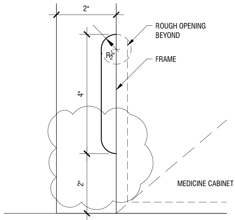
ELEVATION DETAIL
