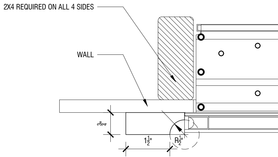
PLAN DETAIL AT FINGER PULL
